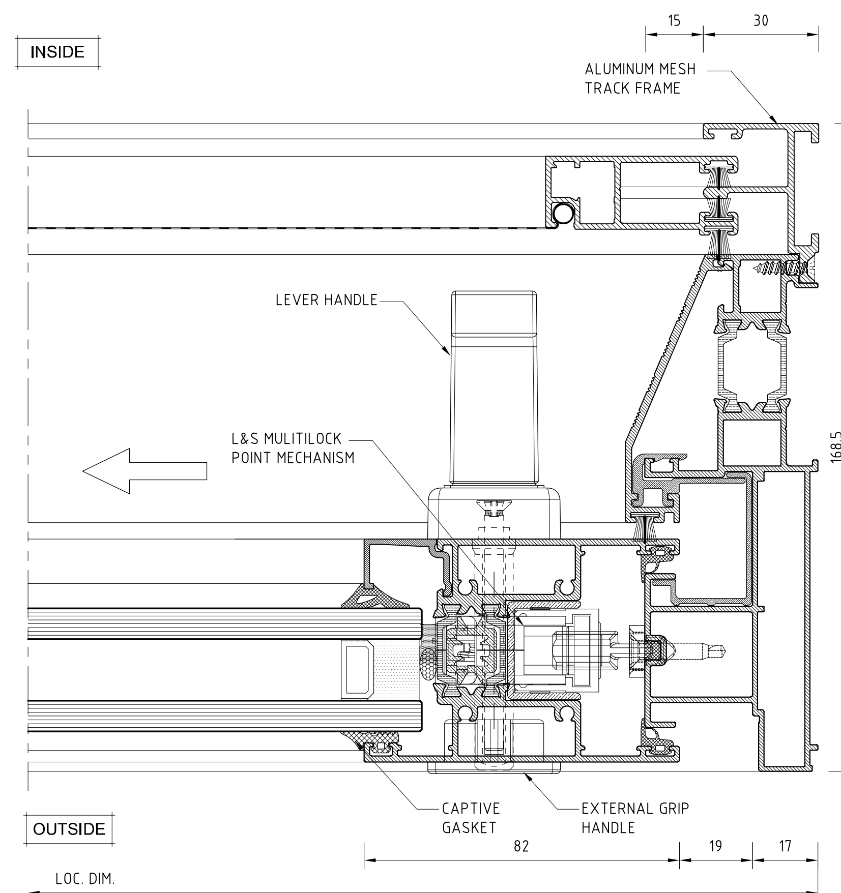
JAMB DETAIL (SLIDING PANEL)
