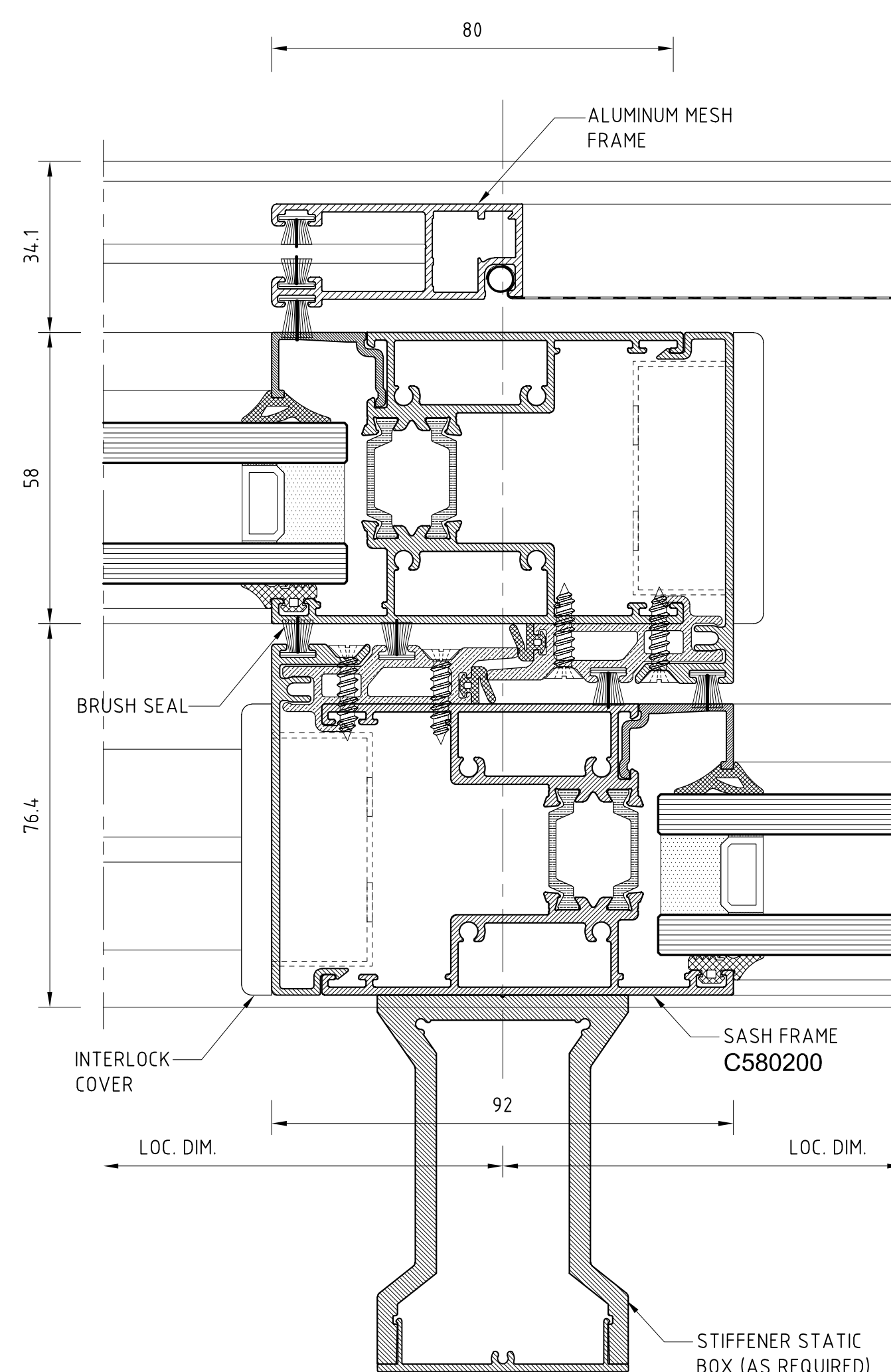
INTERLOCK DETAIL
