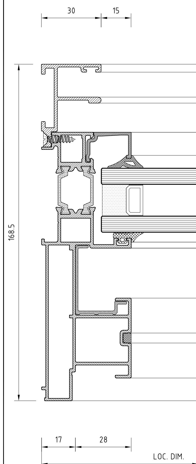
JAMB DETAIL (FIXED PANEL)
